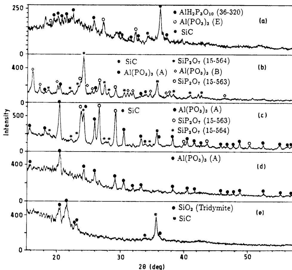
Figure 18 XRD patterns of the SiC whisker block with the undiluted phosphate A12 binder after heat treatment at (a) 200, (b) 500, (c) 800 and (d) 1100 °C (in air) and (e) 1100 °C (in argon).
