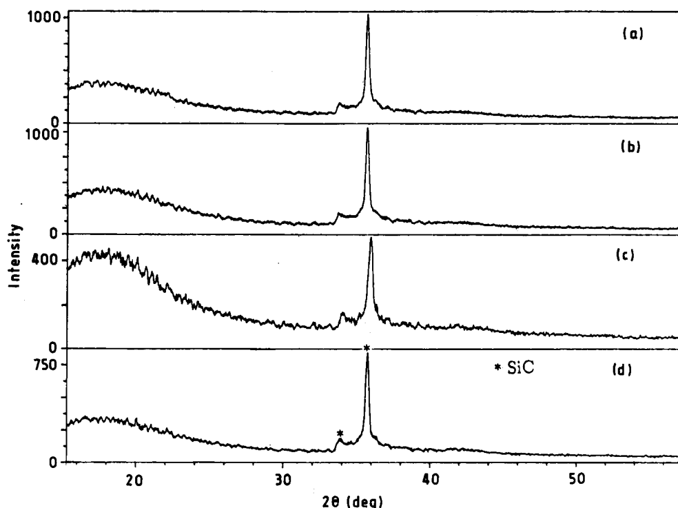
Figure 12 X-ray diffraction patterns from four different points: from (a) the point at the cylindrical edge through two medium points (b and c) to (d) the centre, along the radius of the preform without any binder after heat treatment at 1100°C in air.
