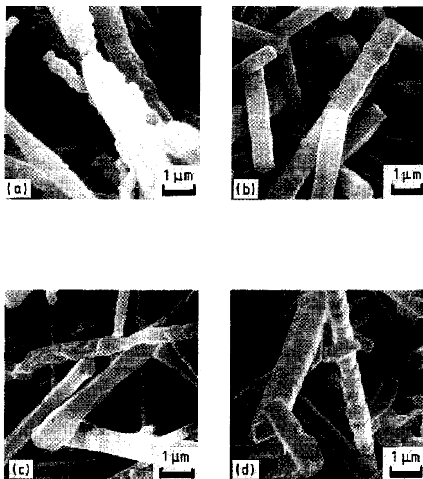
Figure 14 Scanning electron micrographs of the HF-treated SiC whiskers from the surfaces of the preforms made by using (a) the phosphate A23 binder after heat treatment at 1100 °C in air, (b) without any binder, (c) the silica binder at 1100 °C in air, and (d) the silica binder at 1100 °C in argon.
