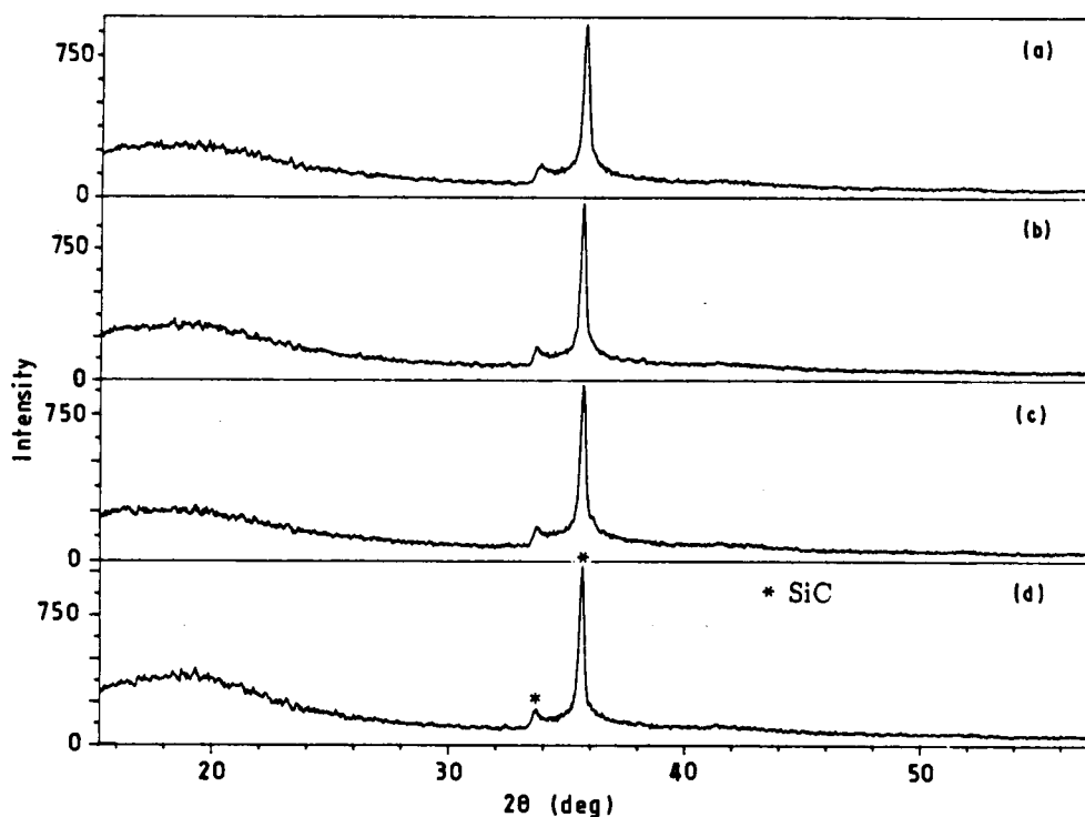
Figure 11 XRD patterns from four different points: from (a) the point at the cylindrical edge through two medium points (b and c) to (d) the centre, along the radius of the preform without any binder after heat treatment at 1100°C in argon.
