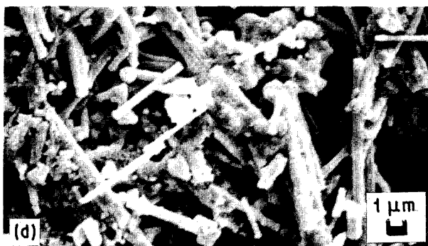
Figure 2 Scanning electron micrographs of preforms with the silica binder after heat treatment in (a, b) air or (c, d) argon at 1100 °C.
